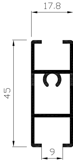
Parteluces vidrio simple Ref: 2108
