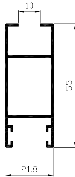
Hoja lateral 55 vidrio simple Ref: 2106
