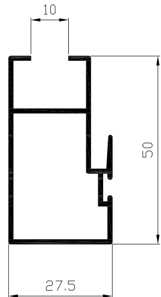
Hoja central vidrio simple Ref: 2105
