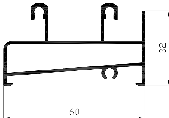
Marco inferior Ref: 2102
