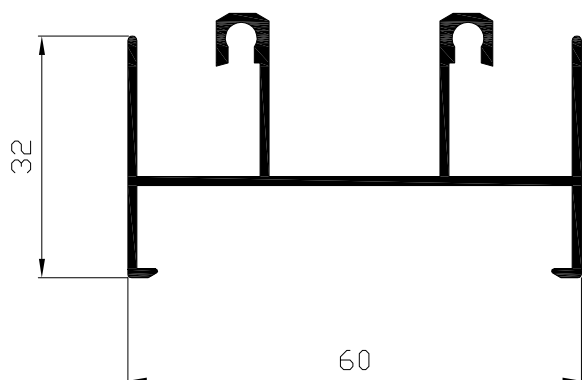
Marco superior Ref: 2101
