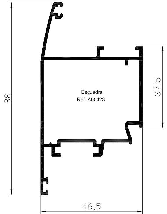
Hoja apert.ext puerta 40 Ref: 4915
