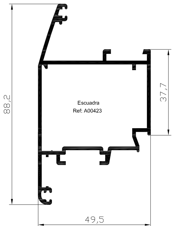
Hoja apert.ext puerta 45 Ref: 5915
