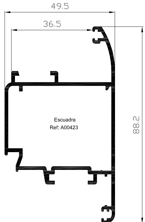
Hoja apert.ext puerta 45 Ref: 4515
