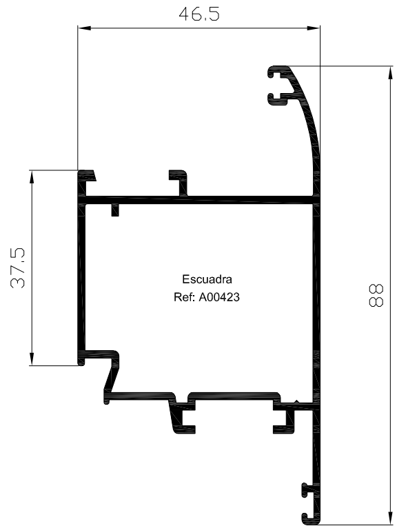
Hoja apert.ext puerta 40 Ref: 4015
