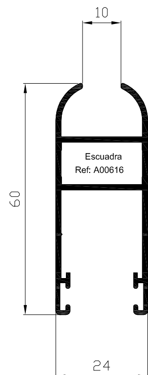
Hoja 60 perimetral H=10 mm Ref: 6104
