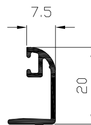
Junquillo curvo c.grapa Ref: 4116
