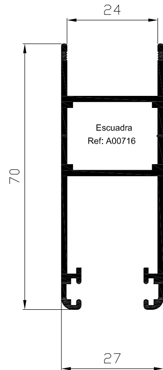
Hoja 70 perimetral H=24 mm Ref: 7124
