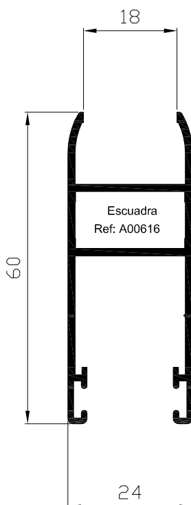
Hoja 60 perimetral H=18 mm Ref: 6114
