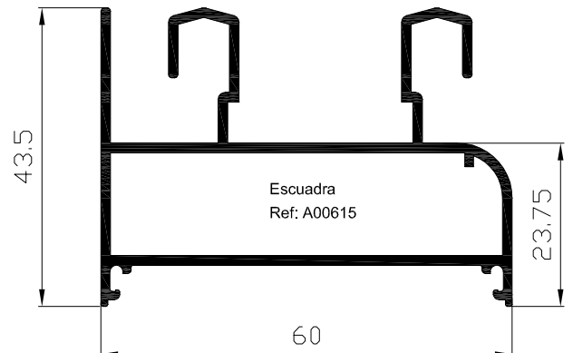
Marco perimetral 60 mm Ref: 6101
