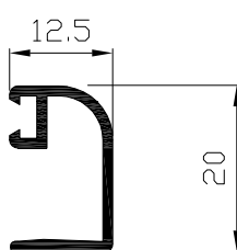
Junquillo curvo c.grapa Ref: 4115
