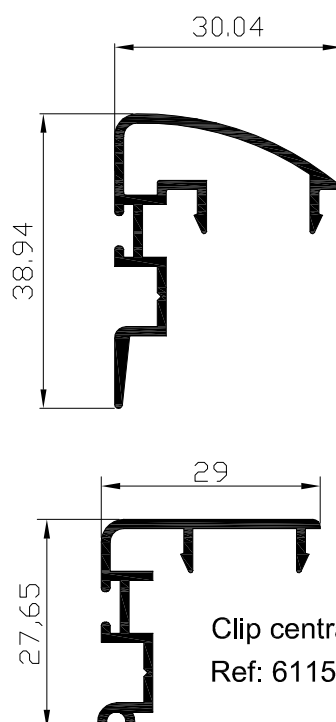
Clip central hoja 60 Ref: 6105
