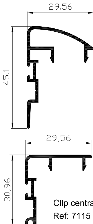
Clip central hoja 70 Ref: 7105
