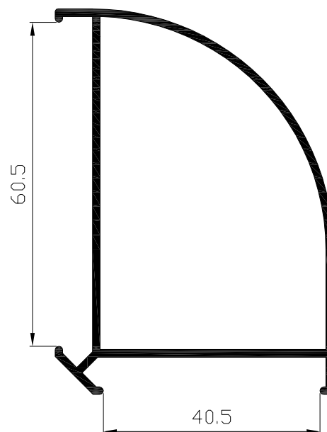
Esquinero 90° corredera SELECT-60-abatible Ref: 2223
