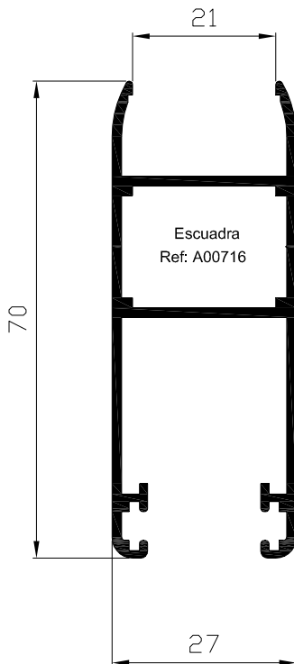
Hoja 70 perimetral H=21 mm Ref: 7114
