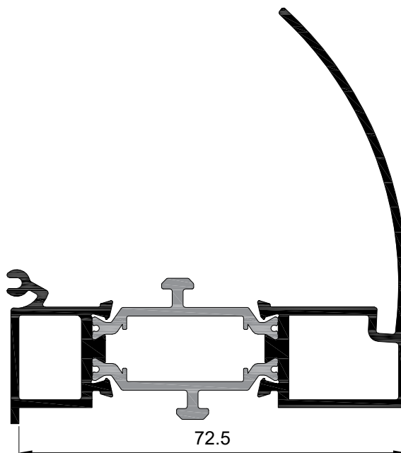
Esquinero regulable macho Ref: 7220
