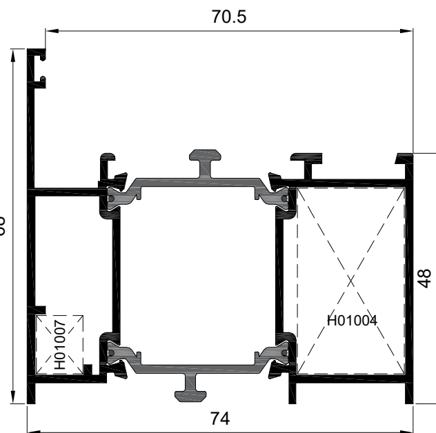
Marco puerta Ref: 7602
