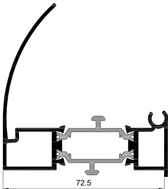
Esquinero regulable hembra Ref: 7221
