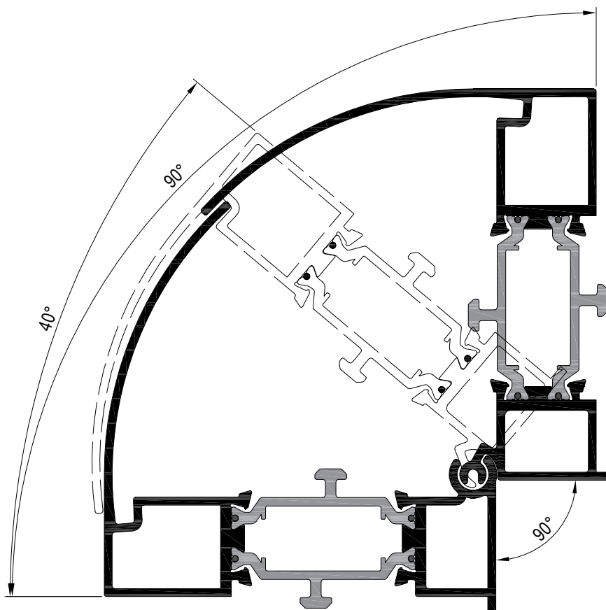
Esquinero regulable hembra Ref: 7221
