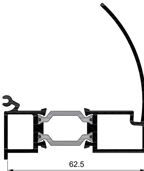
Esquinero regulable macho Ref: 0000
