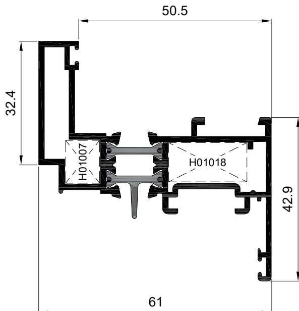
Hoja Ventana Ref: 5504
