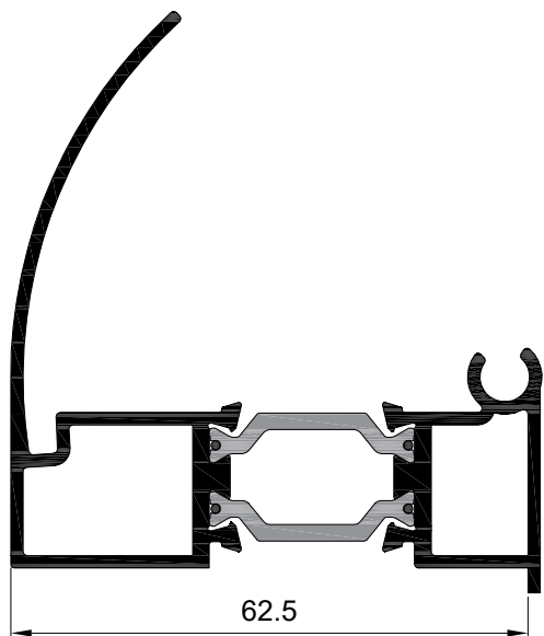
Esquinero regulable hembra Ref: 0000
