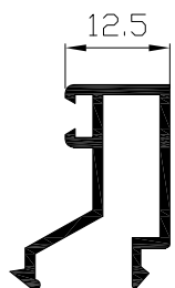
Junquillo recto Ref: 4105
