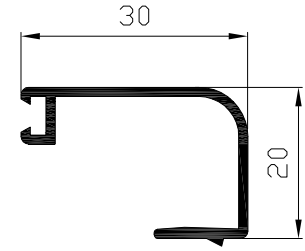
Junquillo curvo c.grapa Ref: 4118
