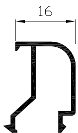
Junquillo curvo Ref: 4124
