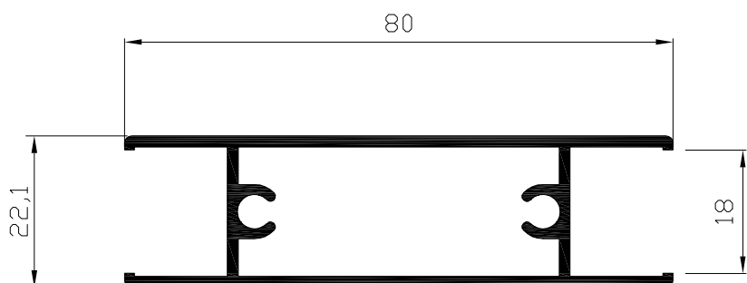
Parteluces H=18 Ref: 9218
