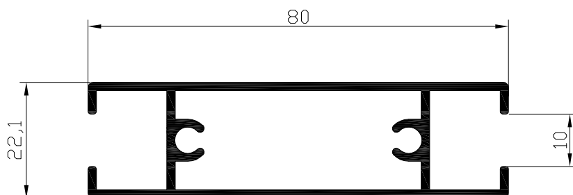
Parteluces H=10 Ref: 9208
