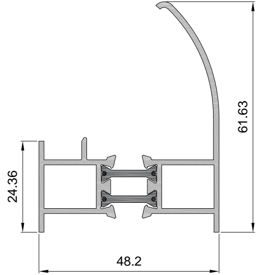
Esquinero regulable hembra Ref: 4822
