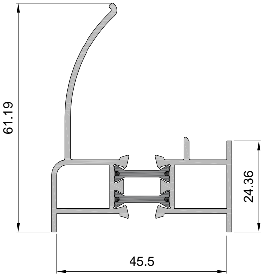
Esquinero regulable macho Ref: 4821
