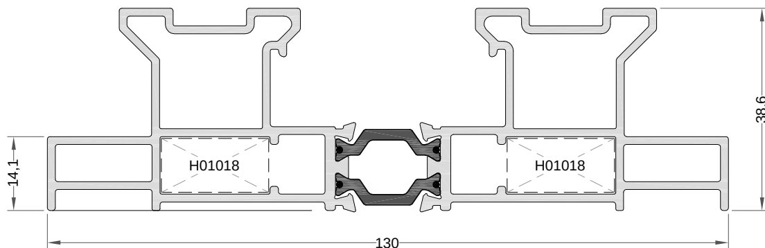
Marco perimetral Ref.: 7901
