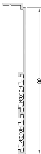
Solape compacto 70 Ref: 8480
