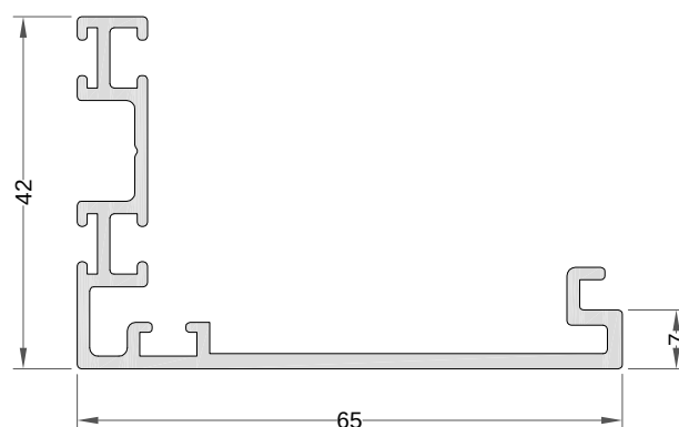
Clip central Ref.: 7905
