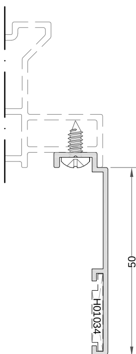
Solape resalte 50 Ref: 9450
