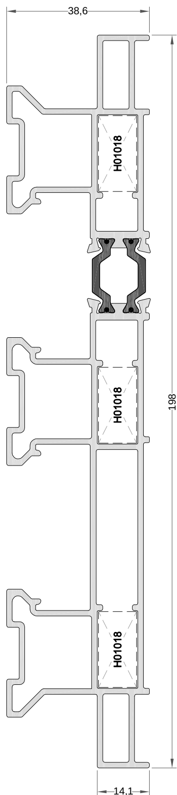
Marco perimetral 3 carriles Ref.: 7931
