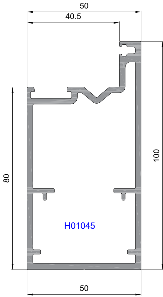
Perfil Corredera Portón Ref:1644
