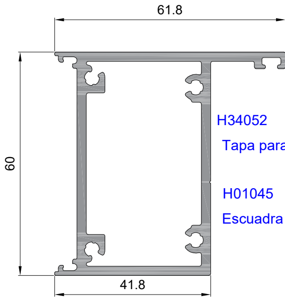
Marco puerta Ref:1642
